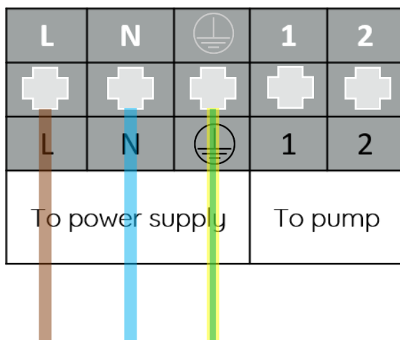
Monophase
